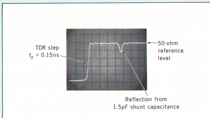
Fig. 1. Oscillogram of typical TDR display showing test step ( t_r = 0.15 ns) and reflection from capacitive discontinuity of about 1.5 pF.
