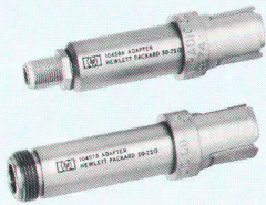
Fig. 1. New -hp- Models 10457A-8A 50-to-75-ohm adapters simplify testing of 75-ohm systems with -hp- Model 1415A Time Domain Reflectometer. Adapters are 25-ohm resistors with one GR874 connector and one type 'N' or 'F' connector.
