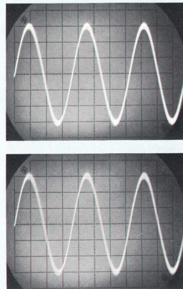
Fig. 2. Oscillograms, made with Differential Amplifier plug-in operating while dc-coupled on most sensitive range (50 \mu V/cm), demonstrate absence of drift over extended periods. Time elapsed between first and second oscillograms was 65 hours but there is no discernible drift in dc level of CRT trace.
