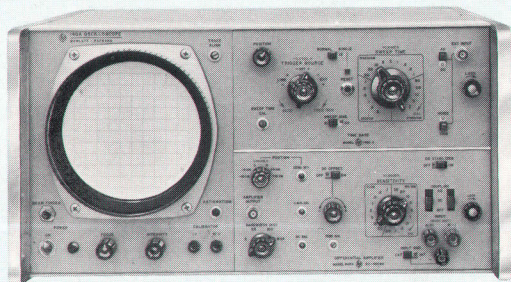
Fig. 1. New -hp- Model 1407A Differential Amplifier Plug-in (in lower plug-in compartment) works with either Model 140A General Purpose Oscilloscope or Model 141A Variable Persistence Oscilloscope. DC stabilization of plug-in amplifier eliminates drift problems, enabling use of dc coupling with deflection factors as low as 50 \mu V/cm. Plug-in has upper frequency limit of 400 kHz.
